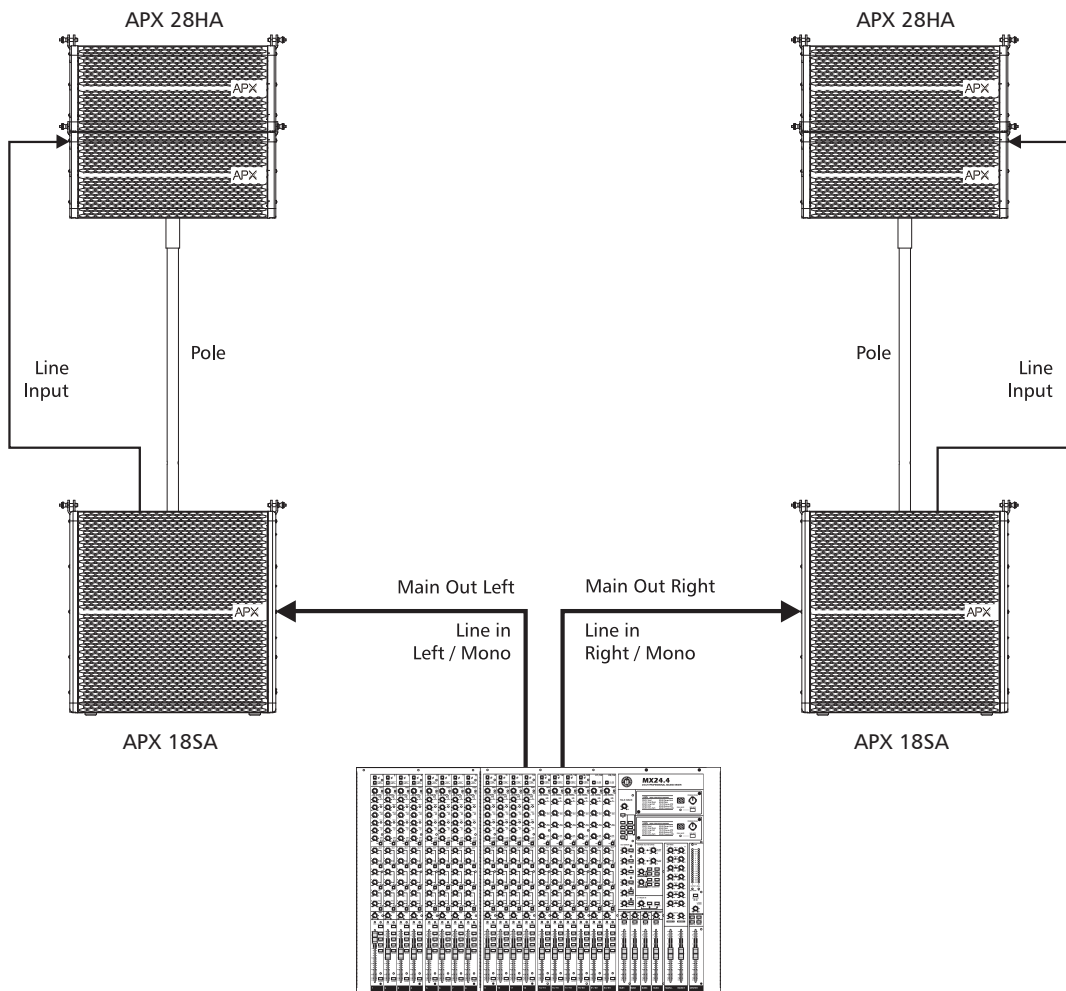
Mixer
